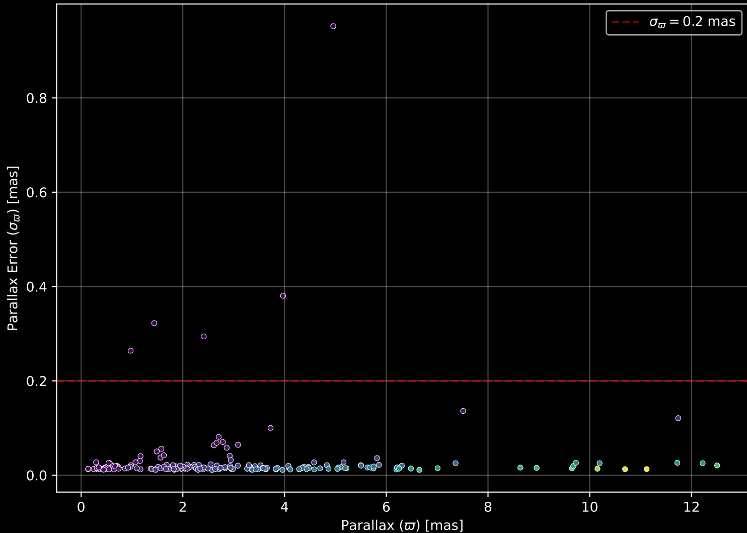
APOGEE DR17 Field: [159+39_MGA] Parallax Quality (n= 178)
