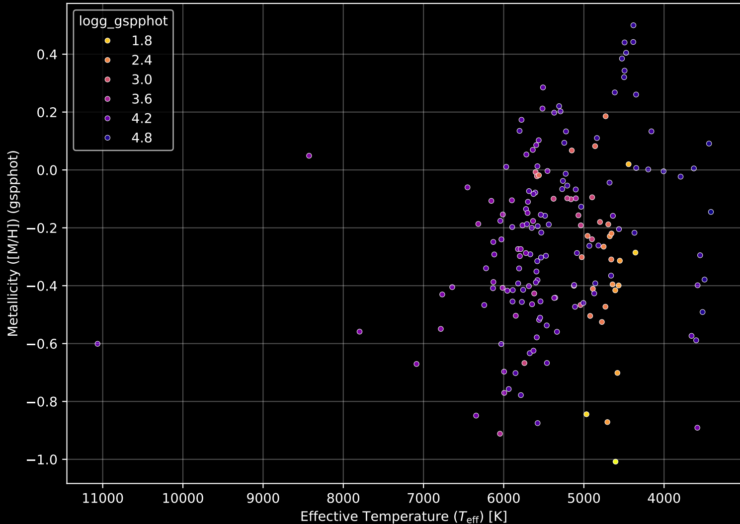
APOGEE DR17 Field: [159+39_MGA] Stellar Population Parameters (n= 178)
