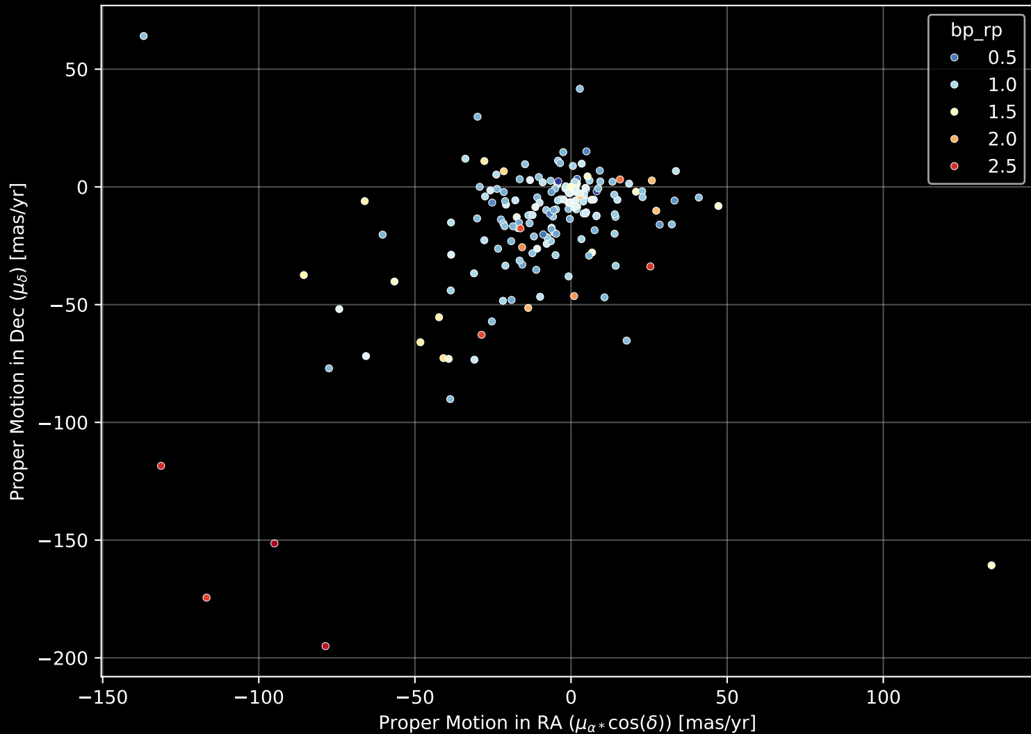
APOGEE DR17 Field: [159+39_MGA] Proper Motion Diagram (n= 178)
