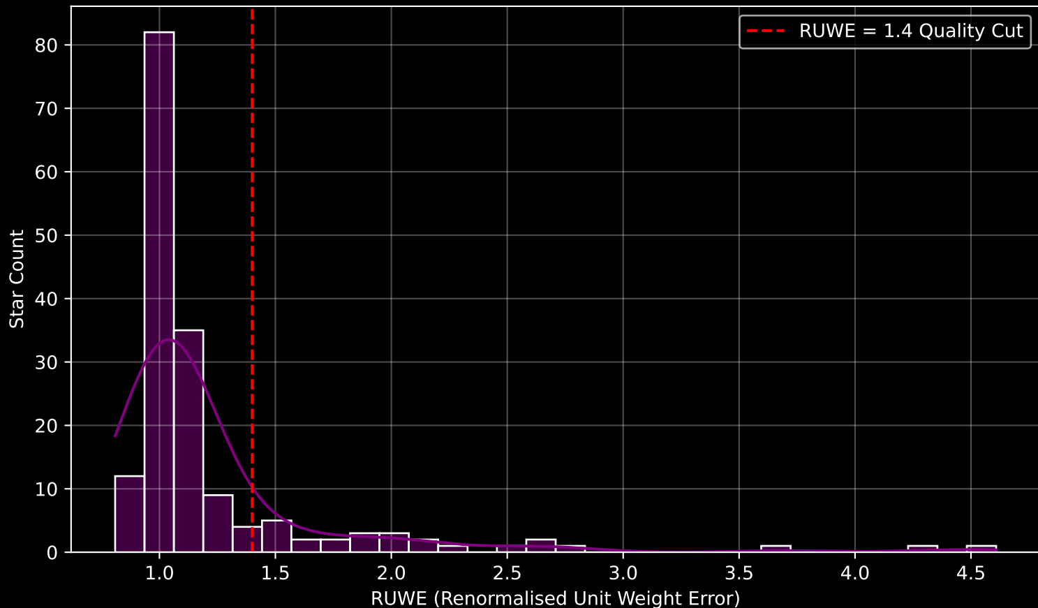
GAPOGEE DR17 Field [159+39_MGA] RUWE Distribution (n= 167)
