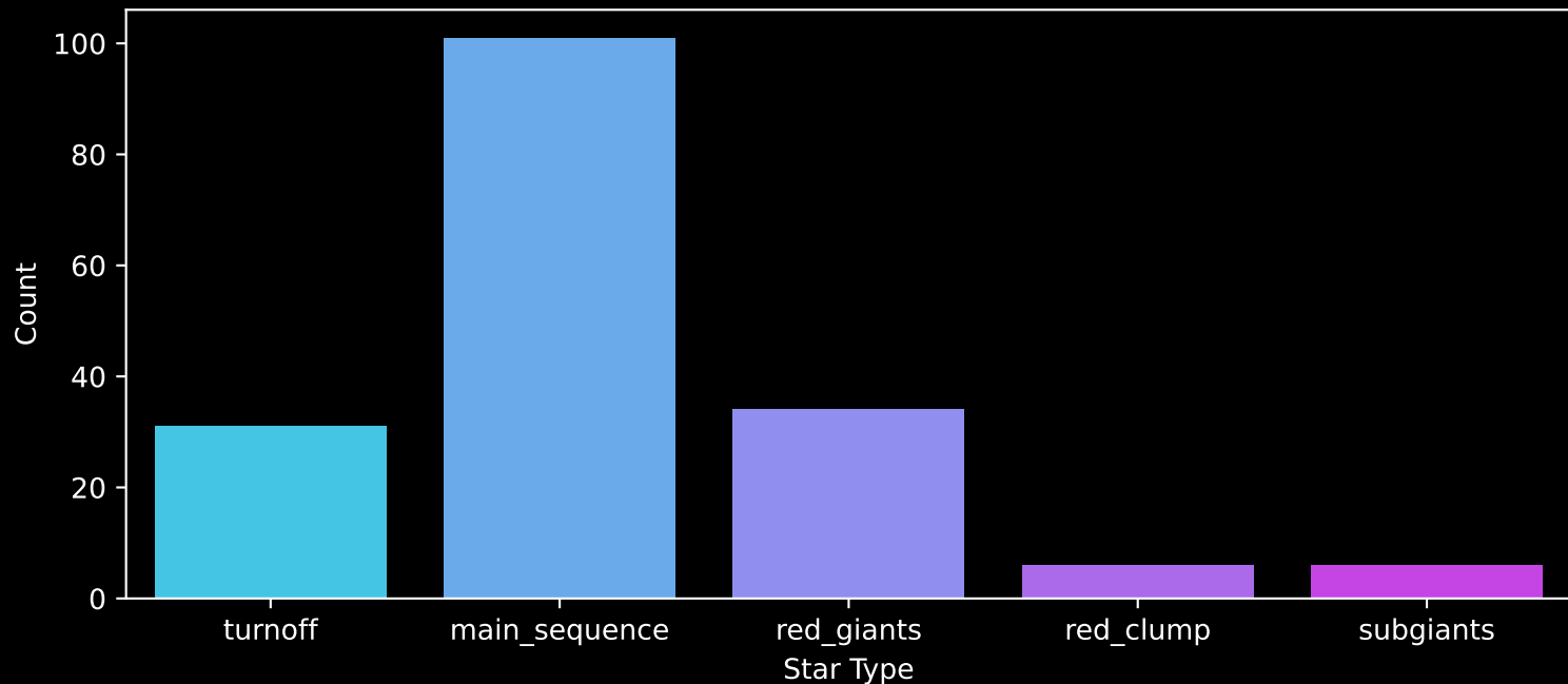
APOGEE DR17 Field: [159+39_MGA] Count plot of Star Type
